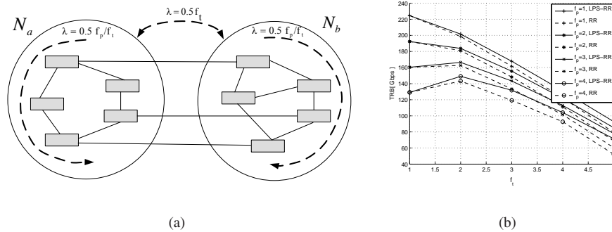
Fig. 1. (a) Network partitions and traffic fluctuation, (b) total residual bandwidth ( TRB ) as a function of f_p and f_t
